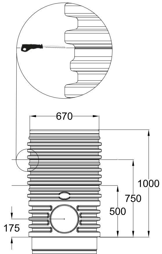
Infiltration connecting piece 1000 DN 600 371015/ 371016
