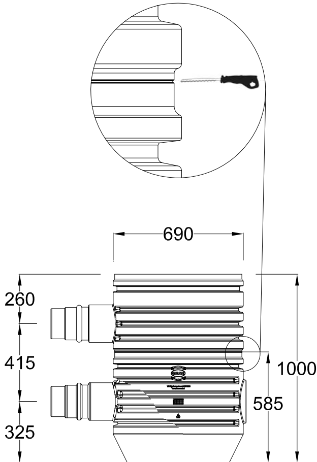
Infiltration distributor module DN 600 330361
